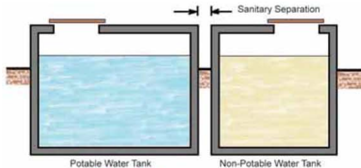
Figure 4.4.3: Sanitary Separation
