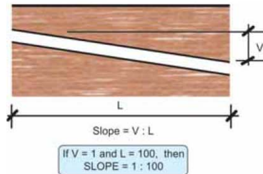
Figure 2.20: Slope
