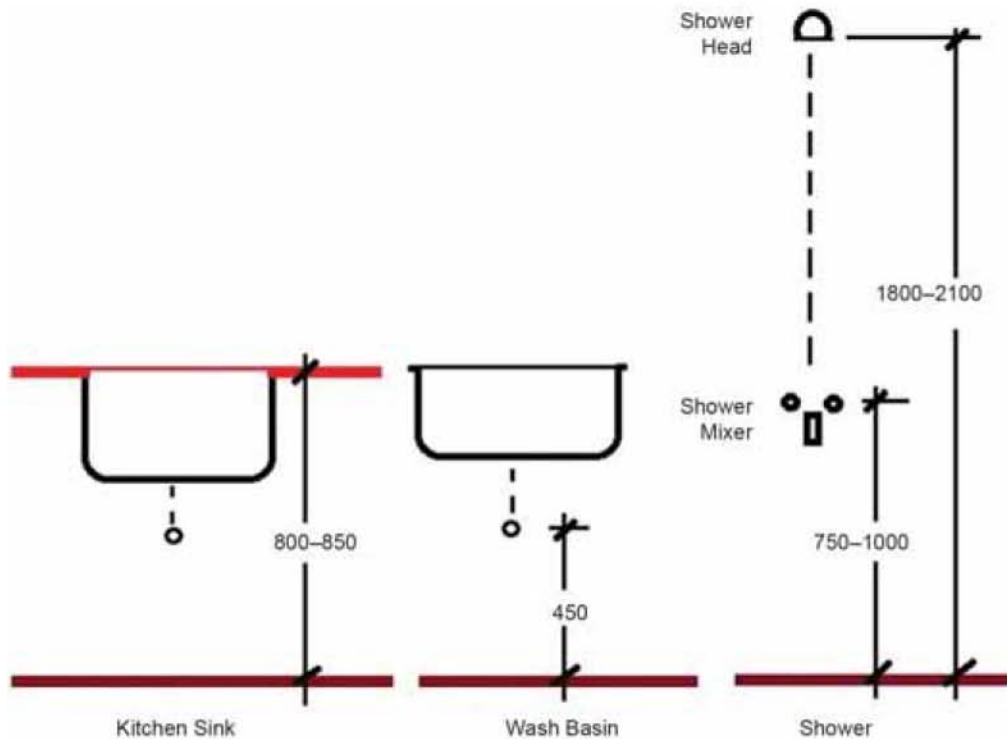
Figure 3.2.8b: Mounting Heights
