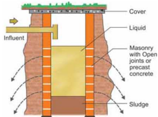
Figure 2.5: Cesspool
