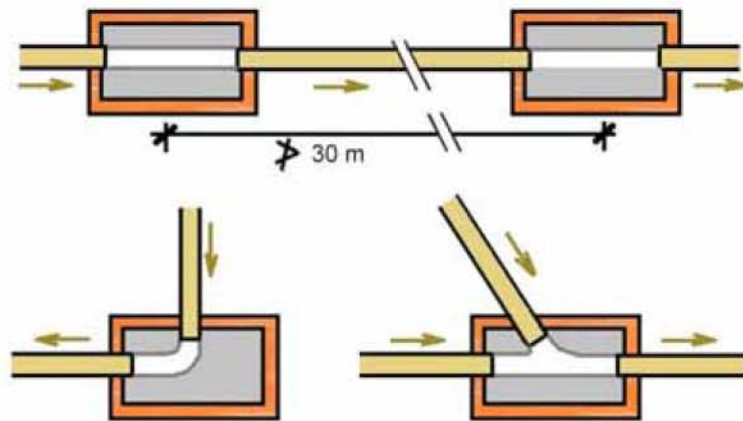
Figure 5.6.2: Inspection Chambers
