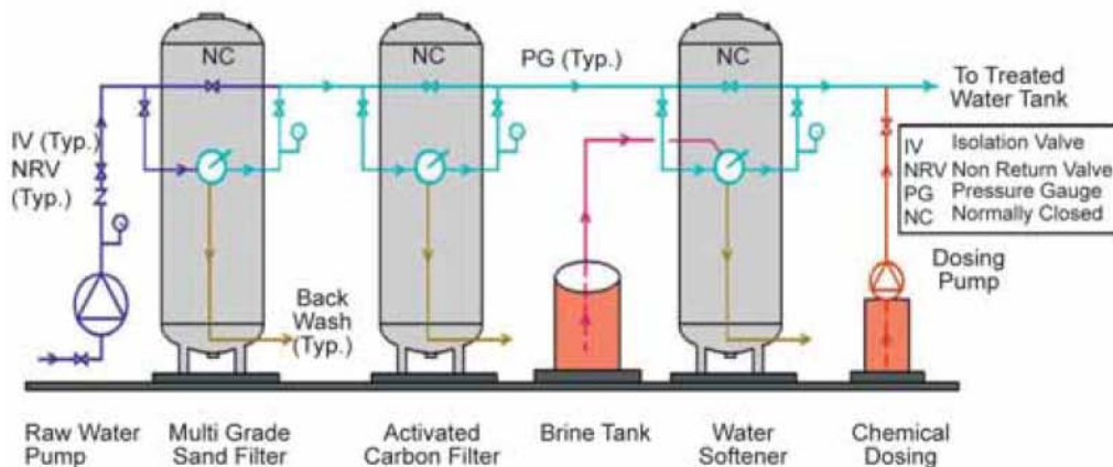
Figure 4.3.2: Schematic-Water Treatment Plant
