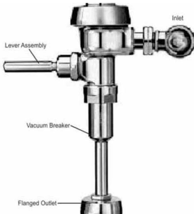
Figure 2.10: Flush Valve
