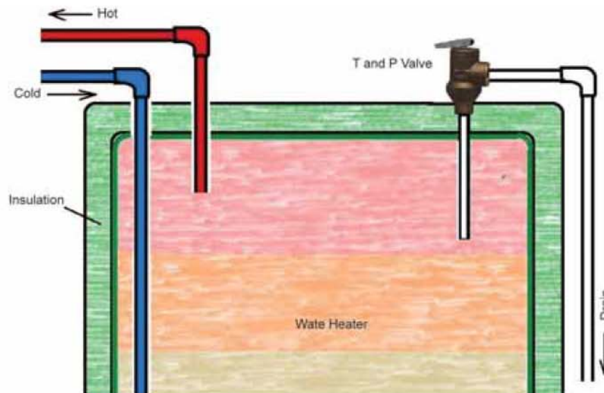
Figure 4.7.4: T&P Valve
