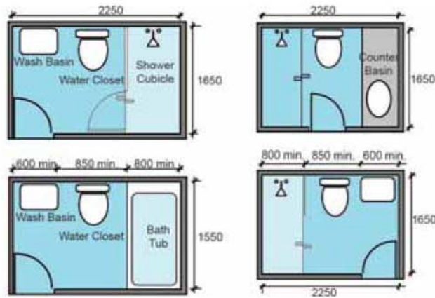
Figure 3.2.5: Washrooms (Alternative Layouts)
