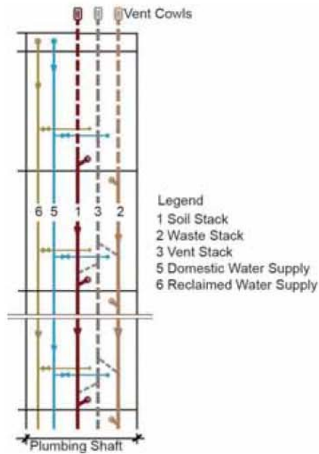
Figure 3.1.3b: Plumbing Shaft-Elevation
